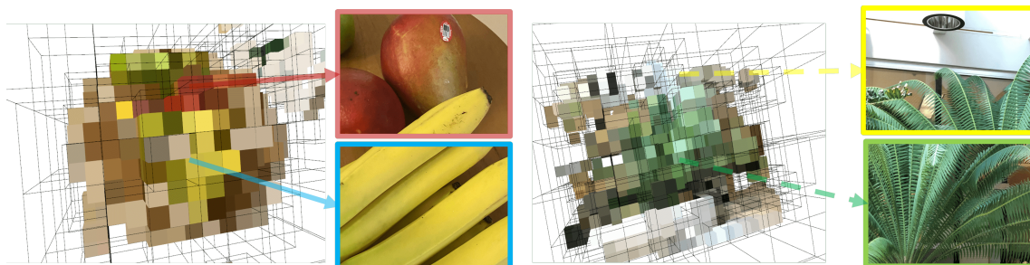
Figure 1: NAScentT jointly optimizes a hybrid explicit-implicit representation consisting of an octree for 3D space partitioning, and structured networks in each active leaf node. Each network maps a spatial coordinate and a direction to a view-independent density and a view-dependent color. NAScentT adaptively allocates more tree nodes to parts of the 3D space with higher scene complexity. Shown here are renderings of novel views from Fruit and Fern.
