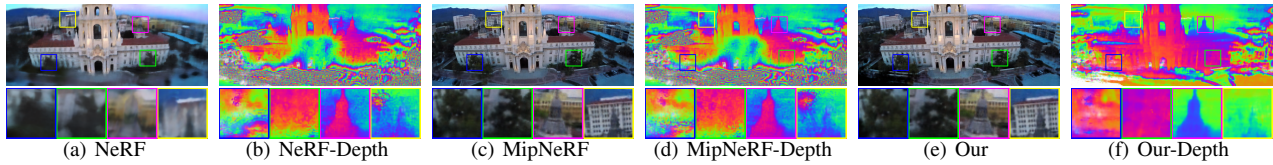
Figure 6: UAV scene reconstruction. We compare our method against NeRF [MST*20], MipNeRF [BMT*21].
