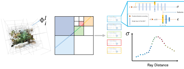
Figure 2: System diagram of NAScenT. The architecture is an explicit-implicit neural representation for the 3D scene, consisting of an octree partitioning of space and a separate lightweight MLP for each leaf node of the octree. The same network architecture and hyper-parameters are used for all octree nodes, which concentrates the model parameters in regions of high complexity. This adaptive representation is combined with an adaptive sampling scheme and differentiable rendering described in the text.
