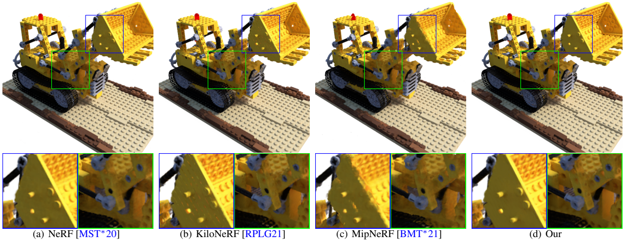
Figure 4: Novel View Comparison on Synthetic Dataset [MST*20]. We render viewpoints from near to far for visualizing viewpoint change and the influence of geometry in rendering.
