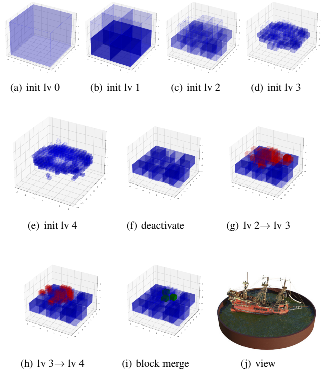
Figure 3: Octree structure update. (a) to (e) show the initial training by using a fully subdivided octree to a given level, with empty nodes culled. (f) only shows active and keep unchanged blocks in level 2, (g) shows block splitting for level 2 to level 3, (h) shows block splitting for level 3 to level 4, (i) shows a block merge to prune the octree for simplification.
