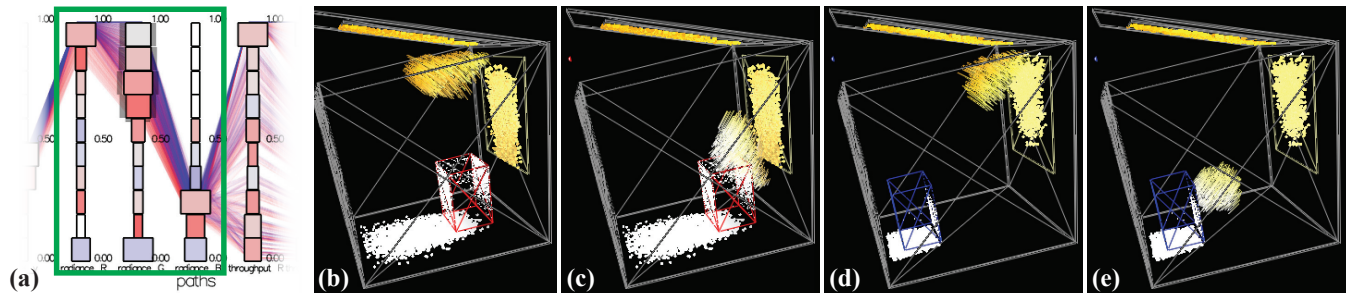
Figure 8: Gizmos can be used to compare two possible candidate positions for a plant. (a) The PCP displays the data associated with each gizmo. The selected paths are visualized and animated in the scene view for the first position in (b) and (c) as well as for the second position in (d) and (e).
