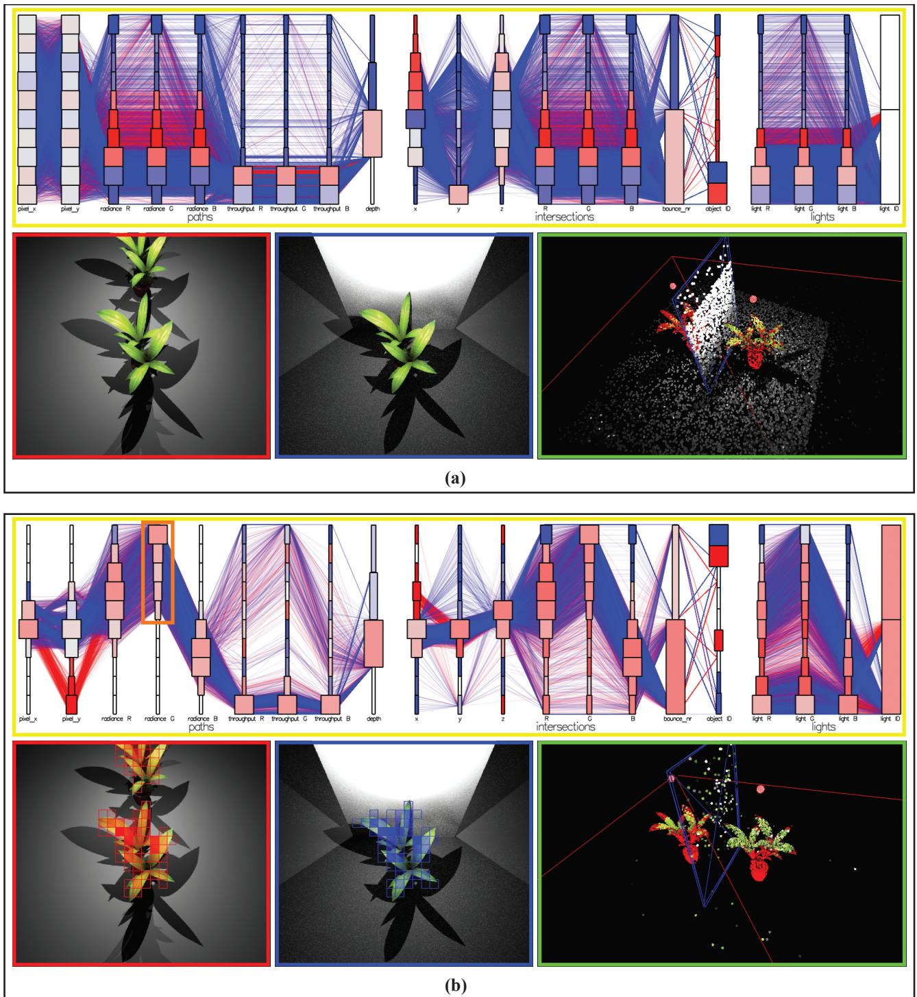
Figure 2: Overview of our visualization tool. The parallel coordinates plot (yellow), the render views (red and blue like the colors in the parallel coordinates plot), and the scene view (green). (a) Visualization of the full data set. (b) Brushing of light paths that have high radiance values in the green component (indicated by the orange rectangle on the axis).
