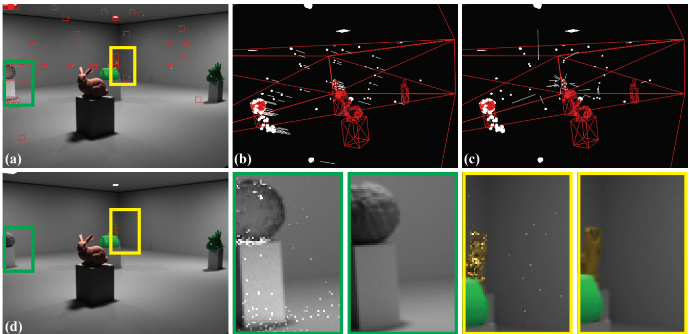
Figure 10: Collecting and animating high-energy paths to determine possible causes of fireflies. (a) The original scene and the selected light paths in the render view. (b) and (c) show the animation of these paths in the scene view. (d) The scene with the changed material in the render view. Close-ups are shown in the bottom right.
