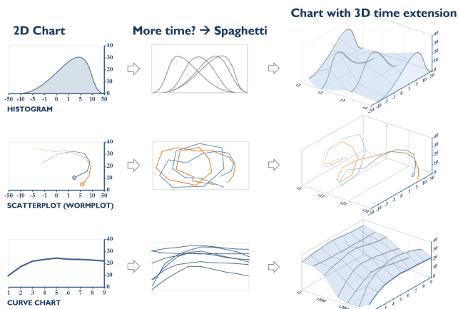
Figure 7: Left: 2D charts without time. Middle: Additional time periods overlaid. Right: Timeseries extended into third dimension.
