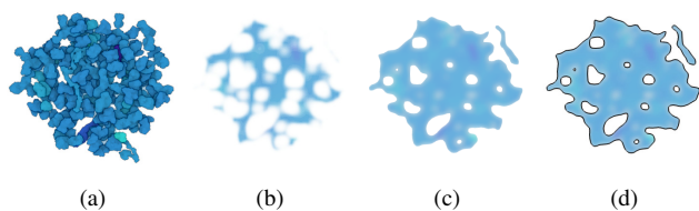
Figure 4: Simplified rendering of molecular data in consecutive steps where the 3D information about the individual molecules is merged into simple geometries. The transition from (a) to (b) shows the blurring with a Gaussian filter. (c) depicts the result after a steep ramp function is applied to the alpha channel to achieve hard edges. Finally, a Sobel operator is applied on the alpha channel (d) to output the display contours of the generated shape.
