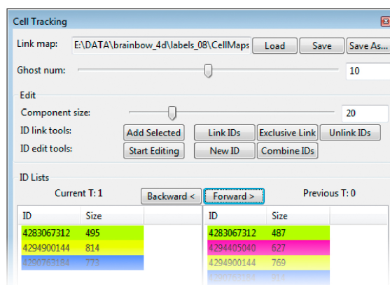
Figure 8: Dialog window for editing cell tracking results. User can load, generate, and save a link map that contains all tracking information. Two sets of tools are provided to edit both tracking and segmentation errors. For tracking errors, IDs can be linked or unlinked; for segmentation errors, a new ID can be generated or several IDs combine into one. IDs of currently selected components are listed in the list. A list of IDs from previous time point is also provided for linking and unlinking. User can also use the Backward and Forward buttons to perform automatic tracking.
