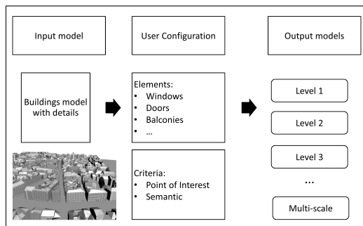
Figure 1: System workflow
