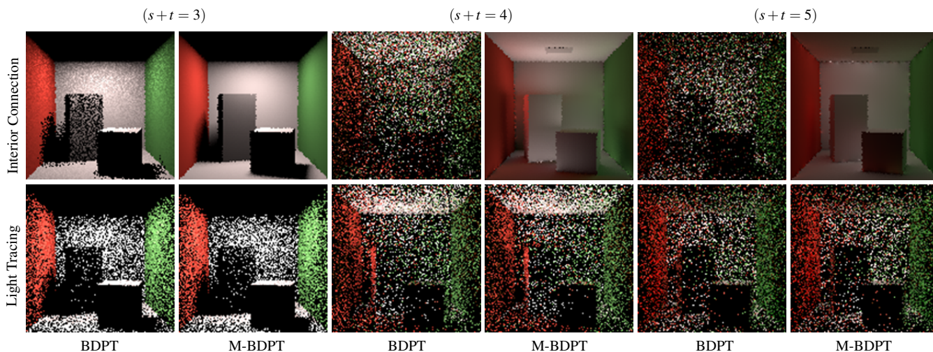
Figure 5: Cornell box scene rendered with BDPT and M-BDPT using different path sampling techniques. Top row: contributions from interior connections ( s \neq 0, t \neq 1 ). Bottom row: contributions from light tracing ( t = 1 ). M-BDPT does not perform better than BDPT for light tracing but it significantly outperforms BDPT otherwise.
