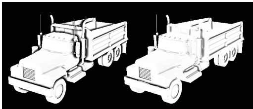
Figure 10: (left) Visible shadow outline in original algorithm. (right) Corrected result with depth range check.
