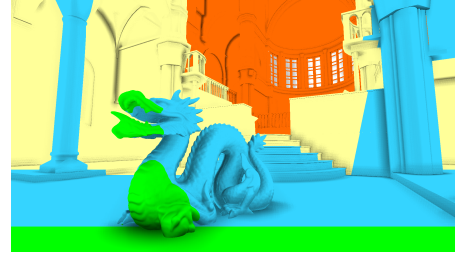
Figure 4: Visualization of the levels of adaptive sampling – back to front: 4, 8, 16, 32 samples.
