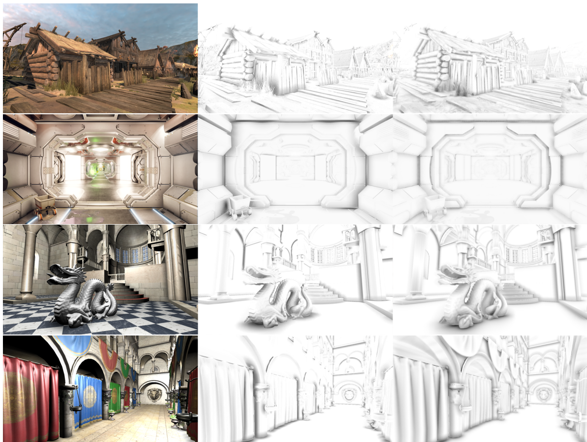
Figure 17: (left) Snapshots of the test scenes (Viking Village, Corridor, Sibenik and Sponza) rendered with VAO++, (center) VAO++ visualization, (right) Unity's built-in SSAO visualization.
