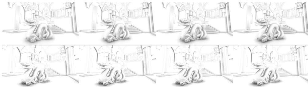
Figure 15: The comparison of Unity SSAO (top) and VAO++ (bottom) for increasing sample counts. For Unity SSAO we used 3, 6, 10, and 16 samples, for VAO++ 2, 4, 8 and 16 samples.
