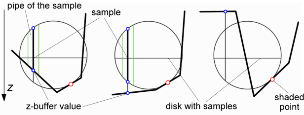
Figure 3: Three possible cases for line samples. Case A: the pipe is partially occluded, Case B: the pipe is completely unoccluded and Case C: the pipe is completely occluded.
