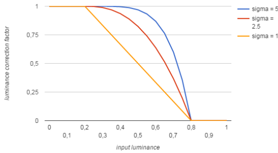
Figure 9: Luminance sensitivity curves for various \sigma (linearity) settings. The threshold was set to 0.5 and width to 0.3.
