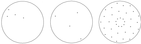
Figure 14: Sampling kernel of size 4 generated by Poisson Disk generator (left). Best permutation of rotations (middle). All rotations (right).
