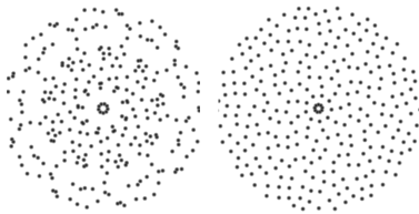
Figure 13: Comparison between the uniform distribution that is rotated afterwards and our modified distribution that considers rotations during generation (16 samples multiplied by 9 rotations).
