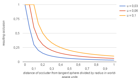
Figure 11: Falloff function describing the thickness of geometry seen by the camera.
