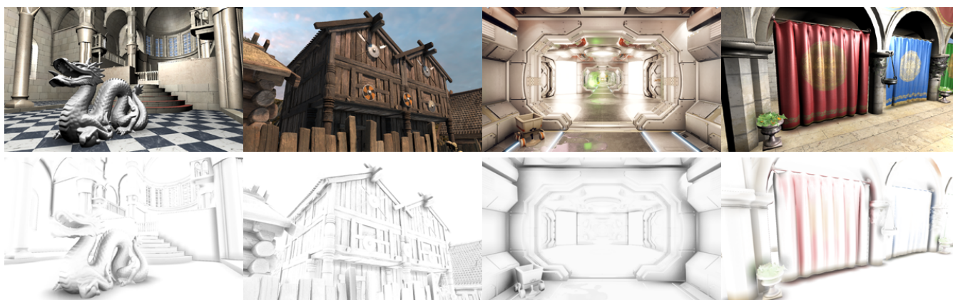
Figure 1: Snapshot of the test scenes rendered in Unity game engine with VAO++ applied (top row) and VAO++ component only (bottom row). The rightmost scene shows VAO++ with color bleeding enabled.
