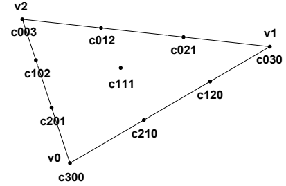
Figure 5: Configuration of control points of a cubic Bézier patch
