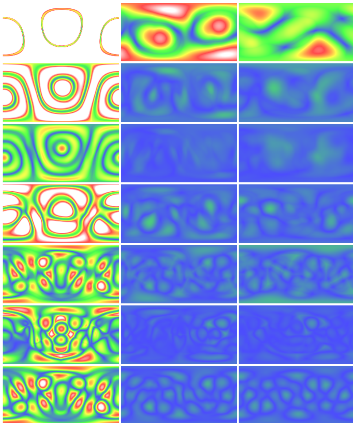
Figure 10: Visualization of the error of the reconstruction of the irradiance environment maps using different bases. top to bottom: 2nd order SH, 3rd order SH, 5th order SH, Ambient Dice with mixture of \cos^2 and \cos^4 lobes, Ambient Dice with cubic Y and linear Co/Cg, interpolated with spherical Bezier patches, Ambient Dice with cubic RGB interpolated with flat Bezier patches, Ambient Dice with cubic RGB interpolated on spherical Bezier patches
