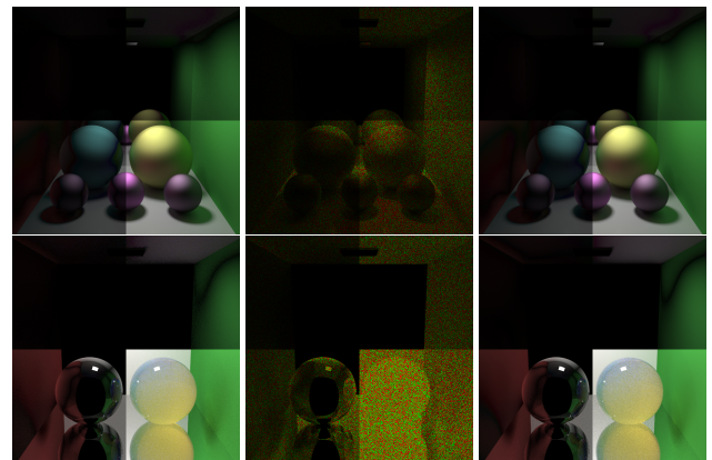
Figure 2: Our bi-directional polarised light transport algorithms converge to the same results as polarised unidirectional path tracing. Each quadrant of the images shows one of the Stokes component, from top to bottom, left to right: S_3 , S_1 , S_2 , S_0 . Left image rendered with PT (top) or VPT (bottom), right image rendered with VCM (top) or VBPT (bottom) and the middle image shows the difference between the two. Top row shows scene glossy and bottom row shows scene glass.
