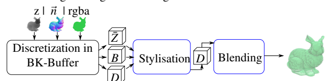
Figure 2: Pipeline used for feature-based stylization with Bucketed K-Buffer. The discretization pass fills the buffer Z , the bucket buffer B and the data buffer D with their respective information (see Section 4). The stylization extracts features and applies modulation on fragment's data (see Section 5). Finally, the blending pass consists in traditional OIT back-to-front composition.
