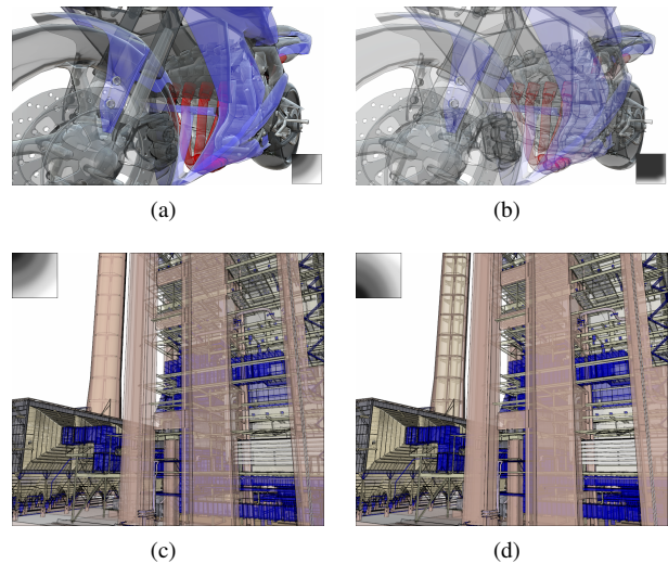
Figure 8: Examples of Mean Curvature Transparency. (a,b) The transfer functions used are respectively the one presented in Figure 7 (45 FPS versus 120 without modulation). (c,d) The transfer functions are shown in the top left corner (10 FPS, versus 20 without modulation). Times are obtained with a resolution of 1200 by 800 for the bike 1000 by 1000 pixels for the UNC Powerplant and 16 layers.
