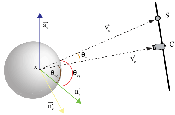
Figure 4: Shading stereo: the normal of \mathbf{x} is adjusted to match the angle of a reference point.
