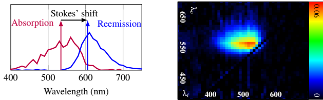
(a) A fluorescent element is often characterised by its absorption spectrum and its reemission spectrum. The offset between the two spectra is called the Stokes shift.
