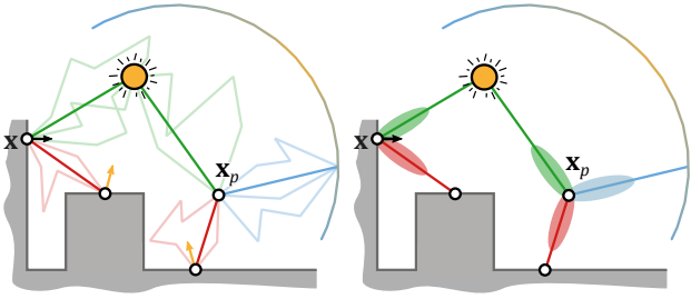
Figure 2: Consider surface \mathbf{x} and probe \mathbf{x}_p locations lit by point (green), environment (blue) and indirect (red) light. Offline rendering traces light paths to solve the radiative transport equation (left; transparent lines). We encode the impulse response of volumetric transport (right), to model media scattering in precomputed lighting.
