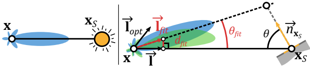
Figure 5: Light scatterd from point (and directional) sources result in circularly symmetric radiance distributions at \mathbf{x} (left; in blue). For differential area sources the distribution skews with the emitters normal and is no-longer circularly symmetric; we determine a best-fit circularly symmetric approximation (right; blue, from green).
