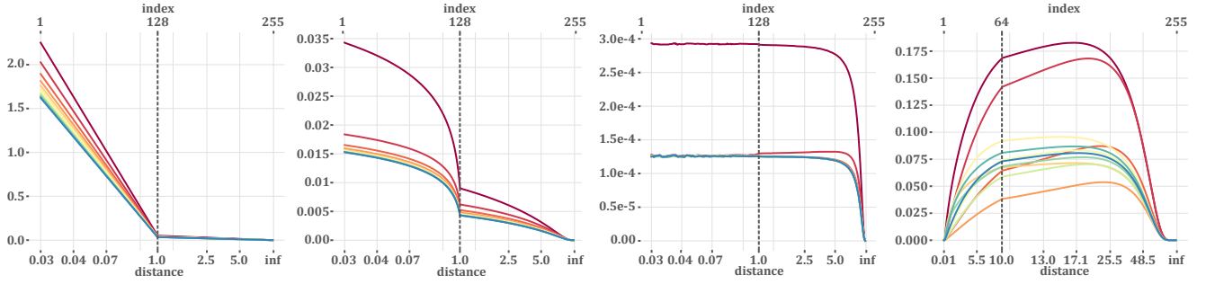
Figure 10: Order-11 ZH response coefficients (dark red to blue) vs. canonical distances d_{\mathbf{x},\mathbf{x}_s} or d_{\mathbf{x},\mathbf{x}_{top}} : 1-, 2- and 10-bounce response for point emitters, and 1-bounce for directional emitters. Table bin indices are on the top x-axis. Radiance tends to isotropy with higher bounces, increasing the ZH DC component (dark red) as expected. Differential area emitter plots (not shown) behave similarly to the point emitter.
