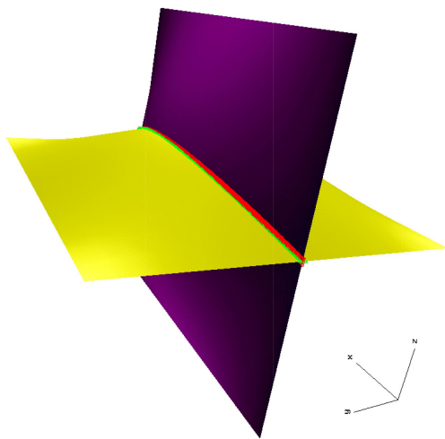
Figure 3: Transversal intersection of two bicubic-Bézier surfaces corresponding to a maximum relative model space error of 0.00350.
