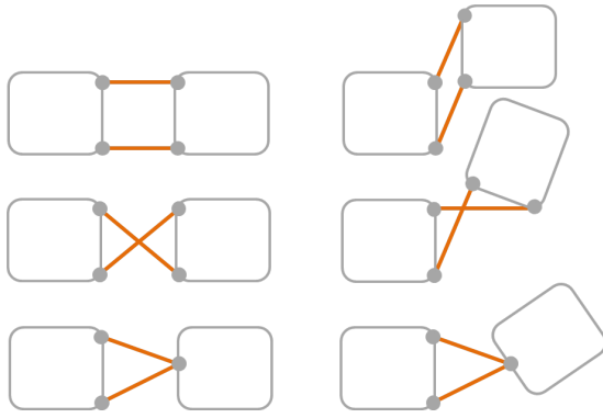
Figure 3: Different ways of connecting two building blocks (from top to bottom): parallel, cross, and pin couplings in their default (left) and deformed configurations (right).
