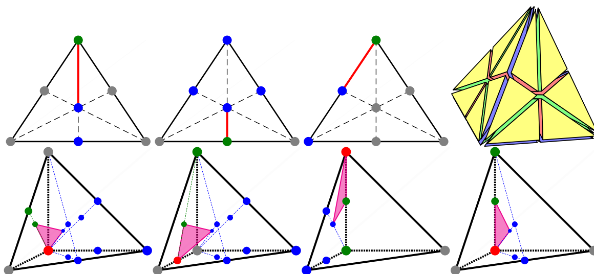
Figure 1: The maximally split configuration in 2D contains three types of cutting flags (top row). The red flag is set if intersections are registered at the green location and one of the blue locations on the triangle. In the maximally split configuration in 3D (top right), each color represents a different type of cutting face, which are shown individually on the bottom row. The correspondence is, from bottom left to bottom right: green, red, yellow, and blue. For each of the four 3D cases (bottom), the shaded flag is set if intersections are registered at the red location, one of the green locations, and one of the blue locations on the tetrahedron.
