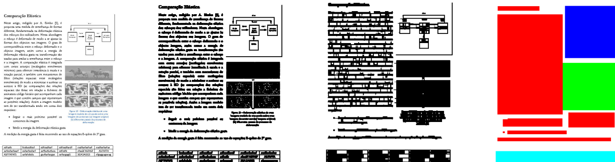
Fig. 4 – Document Analysis Process. Left to right: the original document; the document after thresholding and applying the erosion filter; the result of the RSLA; the final result, with all blocks colored according to their type.
