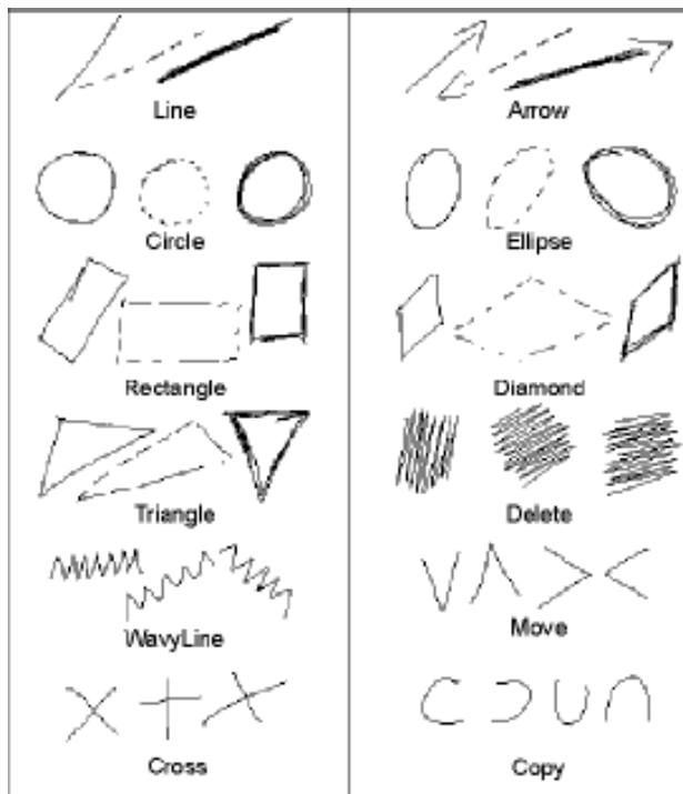
Fig. 2 – Grammar Shapes
