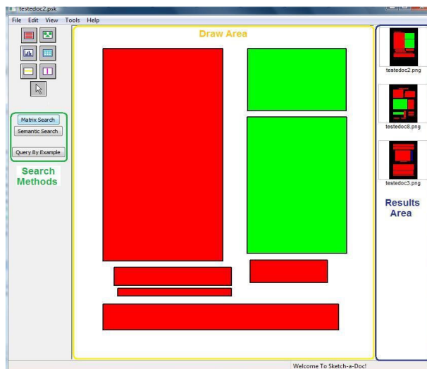
Fig. 1 – Rectangle-based Interface
