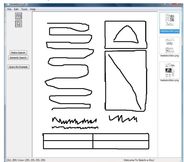
Fig. 3 – Sketch-based Interface
