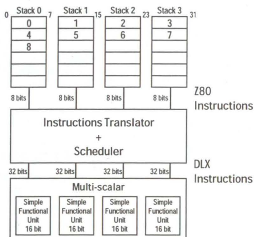
Figure 5-4- Multi-Scalar Architecture
