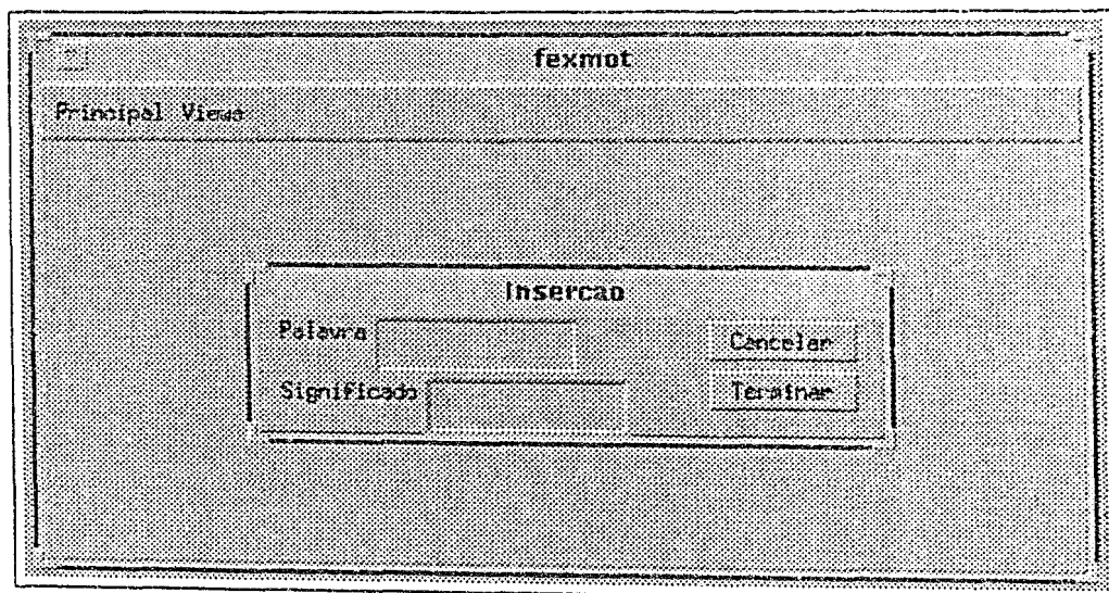
Figura 4: Frontend X11
