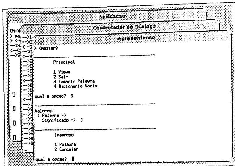
Figura 3: Frontend VT100
