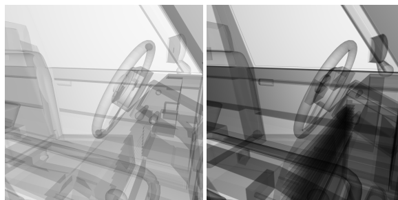
Figure 1: The impact of “losing” intersections at co-planar surfaces with traditional closest-hit kernel and epsilon-offsetting, illustrated using a rendering of the truck model with each surface made partially transparent. Left: rendered with closest-hit and epsilon-offsetting (using a hand-tuned epsilon that just barely avoids self-intersections); right: with a correct traversal kernel that properly finds all surfaces without skipping any. Though the image on the left may look “plausible” in a rendering application it is in fact completely wrong; for a physics-based simulation code this outcome would be quite problematic.
