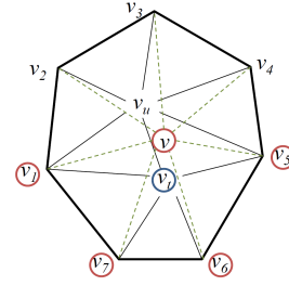
Figure 5: Vertices in the split neighborhood of v_t . The ones used to interpolate the reference coordinate system of v_t are marked in red.
