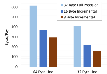
Figure 5: Number of node bytes fetched per ray for the Temple scene using a cache size of 32 kB, with 32 bytes and 64 bytes line sizes. We compare three configurations, namely, a full precision node pair (32 bytes), a node pair with 16-bit plane offsets (16 bytes), and a node pair with 6-bit plane offsets (8 bytes). The bounding planes are shared with the parent node for all configurations.
