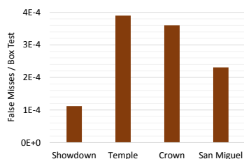
Figure 6: The ratio of false misses to the total number of bounding box intersection tests.
