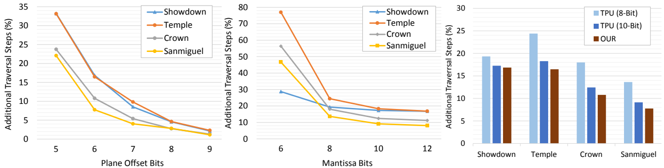
Figure 4: Relative increase in the number of traversal steps with different reduced precision options. Left: our method with different number of bits N_b for the plane offset. Middle: traversal point update (TPU) with 6-bit plane offsets and using different sizes of mantissa bits for the intersection arithmetic. Right: TPU with intersection tests using 8-bit and 10-bit mantissas and our method, both with 6-bit plane offsets.
