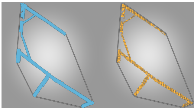
Figure 14: An example for a low-density PR, with density of 13.2%.
