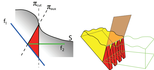
Figure 9: Concave geometry with angle > 90 degrees.
