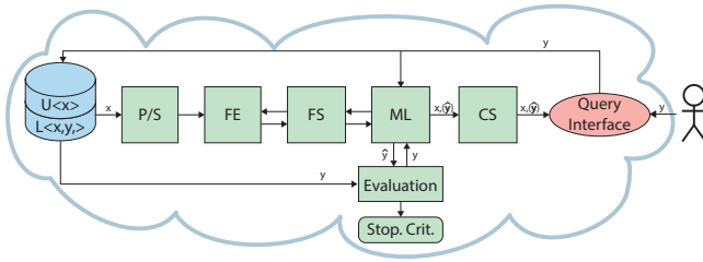
Figure 1: The abstracted AL process. A data source contains unlabeled ( U ) and labeled ( L ) data. Preprocessing, segmentation (P/S), feature extraction (FE), and feature selection (FS) are upstream steps in the process. A learning model (ML) is trained and evaluated as a black-box approach. Candidate suggestion (CS) strategies query new labels y from the oracle which are used to iteratively adapt the classifier until a stopping criterion is met.
