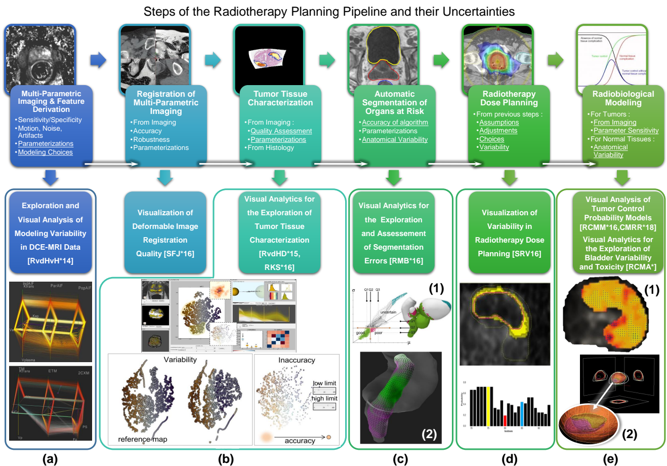
Visualization Strategies Addressing Uncertainty at Each Step of the Pipeline
