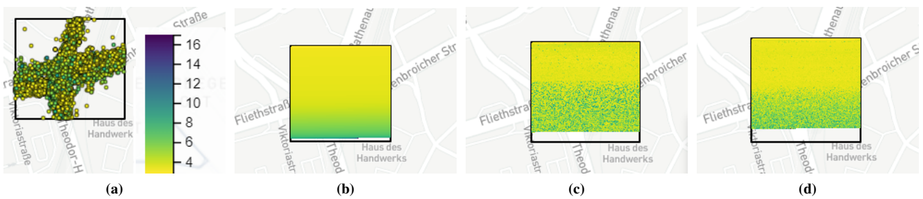
Figure 1: Visualizations of all data points within a certain area around an intersection colored based on their CO_2 emission applying the viridis color scheme [Gar15]. (a) Dot Map of a frequently traveled intersection. (b) Dense-Pixel-Display visualization of the same intersection sorted based on their CO_2 emission. (c) Data points sorted based on their speed. (d) Data points sorted based on their engine speed. The pixels' drawing order within the Dense-Pixel-Displays (b)-(d) left to right and top to bottom.
