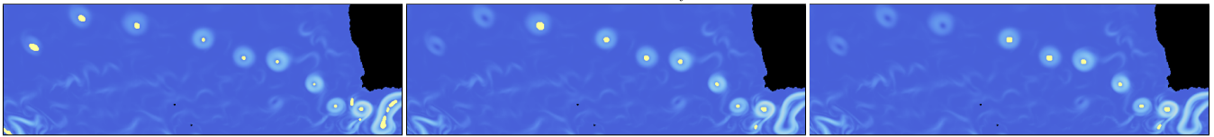
(b) Contour Threshold = 4, Eddies Detected = 14
