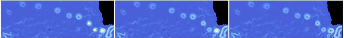
(e) Contour Threshold = 41, Eddies Detected = 3
