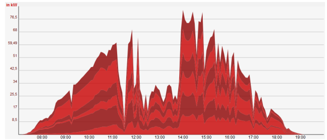
Figure 6: All inverters of a system visually accumulated with alternating colors.
