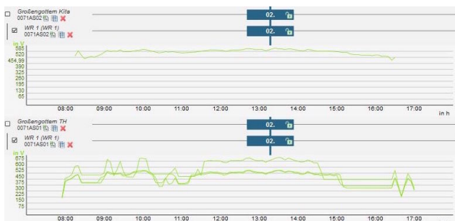
Figure 8: The voltage of the lower power inverters reveal abnormal flanks in the afternoon.
