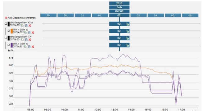
Figure 9: The inverter curves integrated in one diagram allows a more precise comparison.
