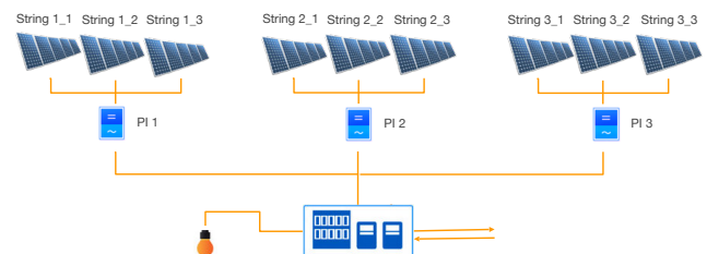
Figure 1: A photovoltaic system. A string is a collection of solar panels. Strings provide DC current to their power inverter, which converts it to AC that is bundled within and fed into the public grid.
