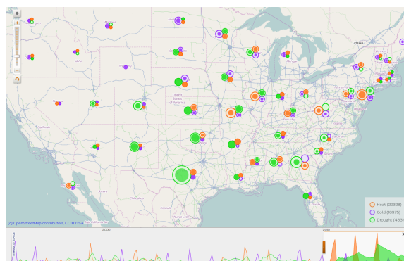
Figure 3: Periods of heat, cold and drought mapped
