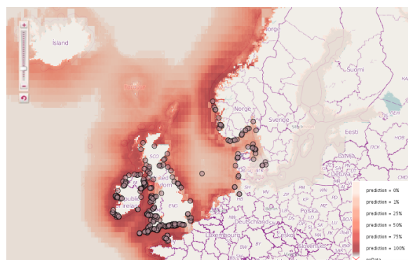
Figure 2: Ecological Niche Modelling Workflow example
