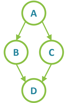
Workflow Graph
