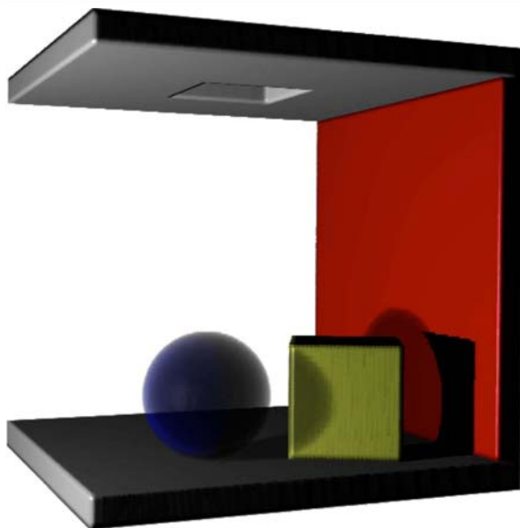
error value of 0.01
