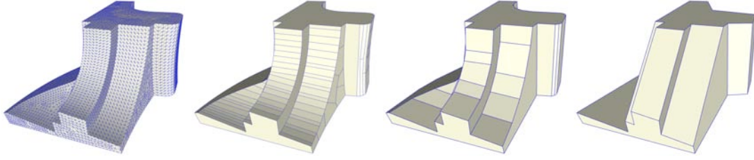
Figure 10.20: A multi-resolution hierarchy of differently detailed meshes that was created by variational shape approximation.
