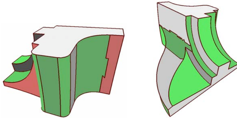
Figure 10.18: Hybrid Variational Surface Approximation: In addition to planes, Wu and Kobbelt also use more general proxies like spheres, cylinders, and rolling ball blends. These proxies allow to recover the semantic structure of the input model.
