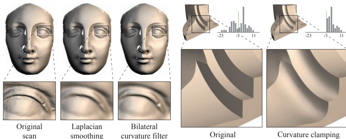
Figure 7.9: Curvature-domain shape processing. The scan on the left has been smoothed using a bilateral filter on the principal curvatures. The fandisk model on the right has been processed by clamping the negative curvatures to obtain smooth fillets for concave corners. The histograms show the distribution of the minimum signed curvature on a logarithmic scale before and after the optimization.
