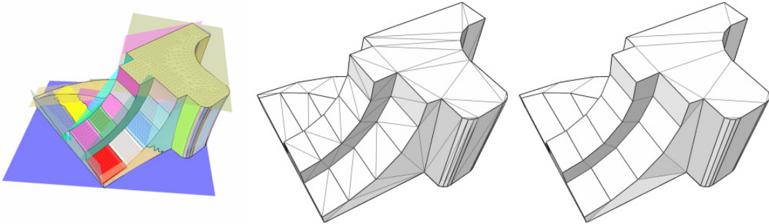
Figure 10.17: Variational Shape Approximation applied to the fandisk model.
