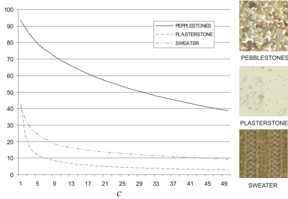
Figure 12: RMS-error of the full BTF-matrix factorization depending on the the number of terms c . There is a direct correspondence between the magnitude and decrease of error and the BTF-complexity.
