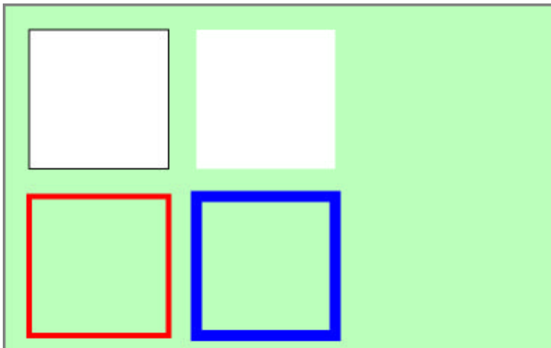
Figure 4.4: Class selection
