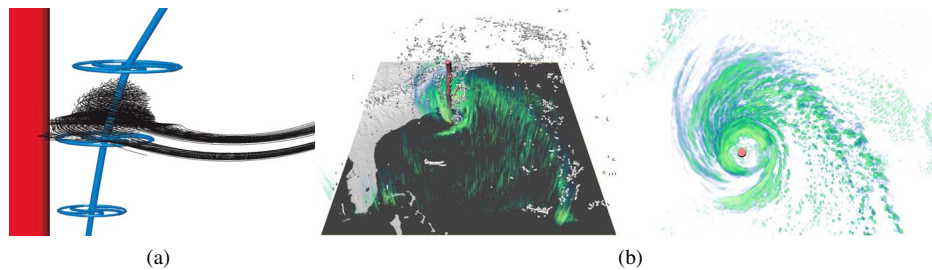
Figure 8: (a) Flow past a tapered cylinder visualized using a non-local vortex detector (image courtesy of Reinders et al. [RSVP]); (b) Visualization of the core of swirling particle motion in the Hurricane Isabel data set (image courtesy of Weinkauff et al. [WST07] © 2007 IEEE).
