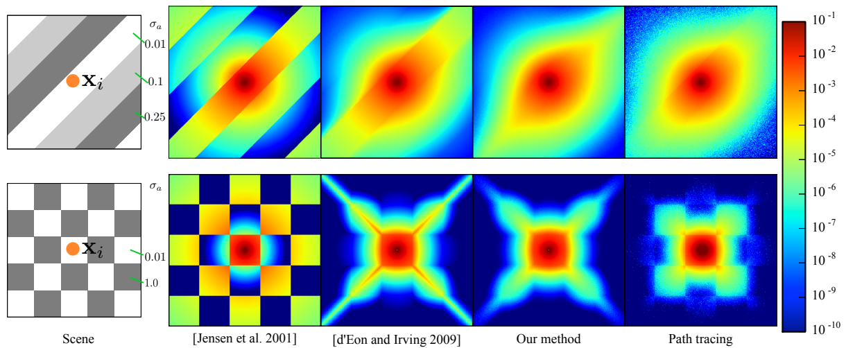
Figure 4: Comparisons with path tracing, a heuristic proposed by Jensen et al. [JMLH01], a heuristic proposed by d'Eon and Irving [dEon09] and our technique. A beam of light enters at \mathbf{x}_i on a nonrefractive semi-infinite medium with the absorption coefficients \sigma_a given by the texture and the constant scattering coefficient \sigma_s = 1.0 . The plot regions are [-15, 15] \times [-15, 15] . Single scattering is excluded for all the results.
