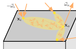
Figure 1: Conceptual illustration of our method. Our method takes optical properties in wide range (shown in yellow ellipse) into account. The range is decided with path integral approach proposed by Premože et al. [PAT*04], which enables us to predict how wide the beam of light will spread in heterogeneous media. We use the average coefficients within this range as the input to a homogeneous BSSRDF model.
