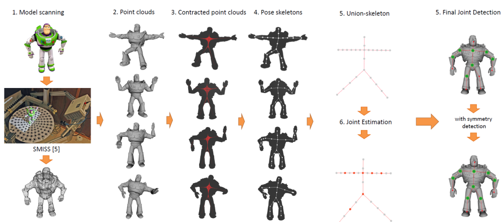
Figure 1: Workflow of our system: from scanning of input articulated model to final detection of its joints.
