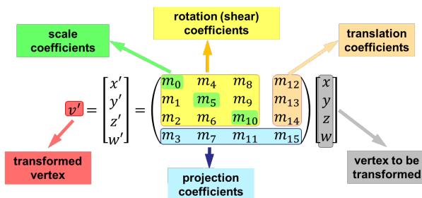
Figure 3: An affine and a projection transformation matrix.
