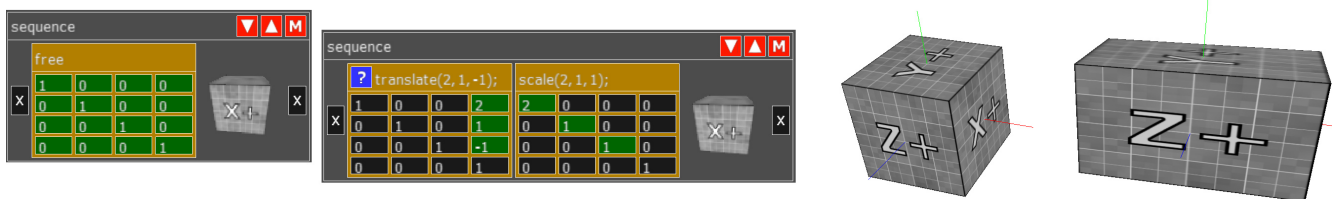
Figure 1: The user of our I3T framework can interactively modify the transformation matrices (left) and immediately see the result in a 3D scene preview (right). The left sequence shows the application of identity matrix and the right sequence is an application of translation and scale. The right-hand side shows the effect of these transformations on a user-defined object.
