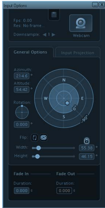
Figure 9: Plugin options.
