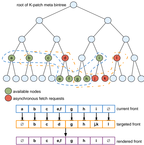
Figure 7: Asynchronous fetching.
