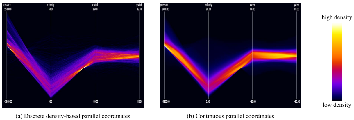
Figure 8: Discrete parallel coordinates computed using the binning approach as described in Section 3.1.6 and continuous parallel coordinates for the “hurricane Isabel” dataset at a spatial resolution of 25 \times 25 \times 5 . A single peak with fast falloffs on both sides is visible at low velocities in continuous parallel coordinates, whereas the discrete version suggests two peaks. The high-density region at low pressure and low velocity constitutes the eye of the hurricane.
