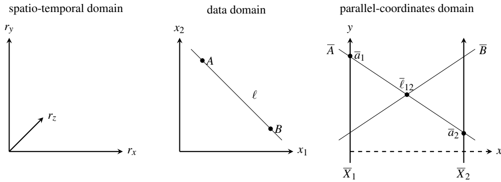
Figure 2: The notation used for different domains. The spatio-temporal domain (left) describes events in space and time with up to 4 dimensions. Many datasets describing abstract data are defined in the data domain (middle) with a finite number of dimensions. The parallel-coordinates domain (right) refers to the xy -plane in Cartesian coordinates that is used to construct a parallel-coordinates system. See Section 2 for an explanation of the point–line duality illustrated above.
