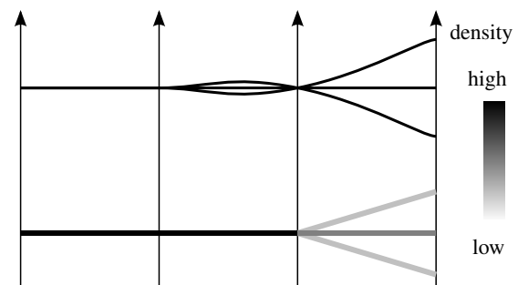
Figure 9: Some ambiguities cannot be resolved entirely using curves (as in Figure 13), because tangents only depend on adjacent axes. The lines appear as one in the leftmost segment using curves (top). The density representation (bottom) reveals two different densities, where the horizontal line appears darker than the other two. Assuming equal and constant densities for each sample, this means that at least two samples are contributing to the density of the horizontal line. In conclusion, the plot must be showing at least four samples instead of three as the top plot suggests.
