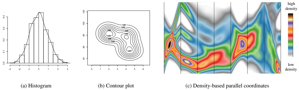
Figure 6: Density visualizations for (a) univariate, (b) bivariate, and (c) multivariate data. The histogram shows a density estimate with discrete bins and an overlaid continuous density estimate reconstructed using a Gaussian kernel. The contour plot for bivariate data shows isolines for a density estimated from point data using a 2D Gaussian kernel. Density-based parallel coordinates are computed from pairs of 2D density fields. A colormap was applied to the density in parallel coordinates.
