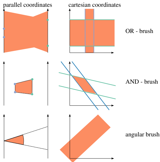
Figure 10: Brushing in parallel coordinates. Top: Axis-aligned brushing. A brush on one axis (e.g. left axis, bounded by the blue points) corresponds to a one-dimensional interval brush in the data domain (bounded by the dual lines). The union (OR) with another interval (green) results in the orange brush. The intersection (AND) of two intervals is shown in the center. Translating the blue and green points in parallel coordinates results in a rotation of the dual region in Cartesian coordinates. The bottom row illustrates the dual of an angular brush to the data domain, which corresponds to a set of ideal points \bar{\ell}_\infty as in Figure 4.
