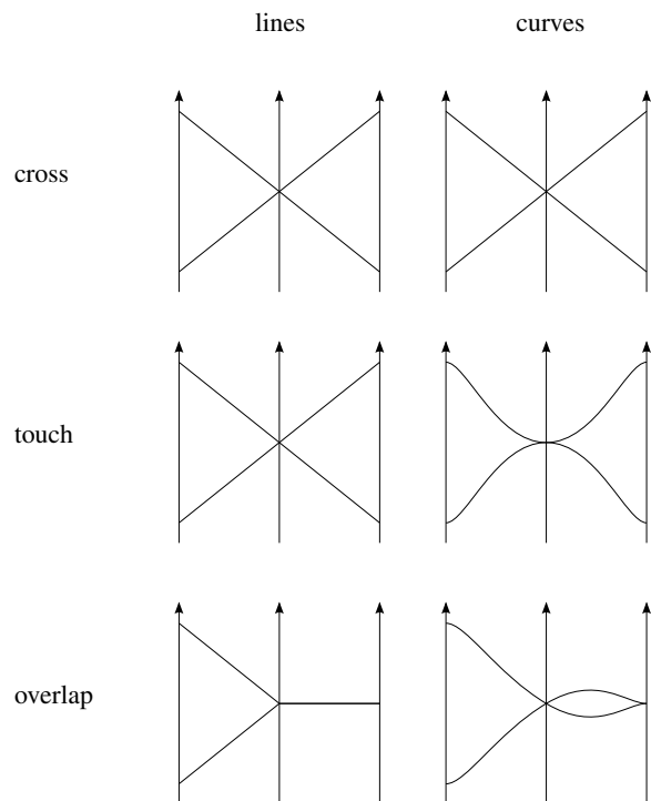
Figure 13: Ambiguities for tracing lines can partly be solved using curves instead of lines. For a pair of lines crossing at the midway axis (top), the curve model exhibits the same pattern. If lines touch instead (middle), a different pattern emerges. Note that without knowing the underlying model, it is still not possible to visually trace the lines. For lines that coincide (bottom), a smooth representation succeeds in disambiguating the samples.
