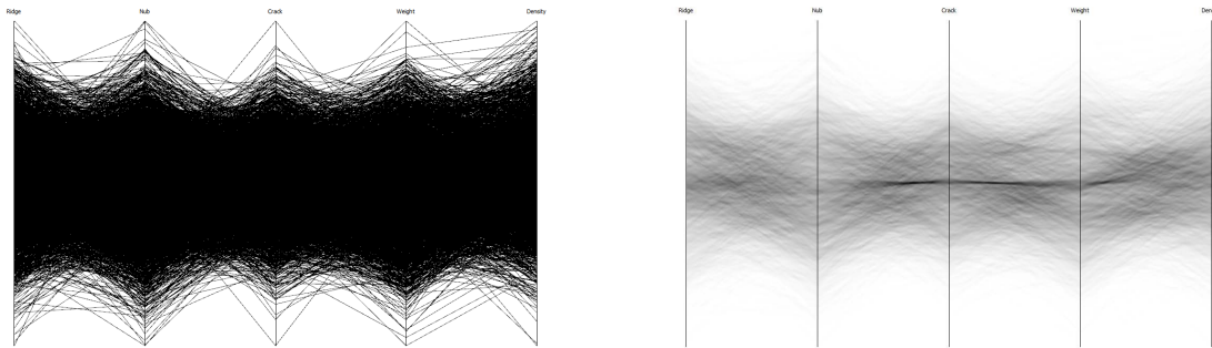
Figure 11: A frequently used synthetic dataset for parallel-coordinates plots about the geometric features of pollen grains. The large number of lines (3 848 observations, left) may hinder the perception of patterns in the data. Note, however, that the hyperbolic shape of the envelope hints at normally distributed data. Density-based approaches (right) may reveal patterns that are not visible otherwise. The cluster of samples that appears in the center forms the word “EUREKA” if viewed in a scatterplot.
