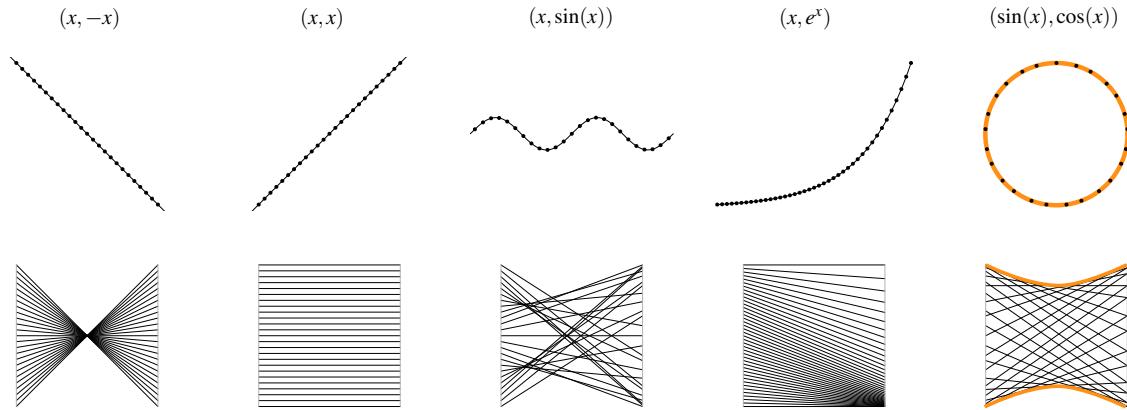
Figure 5: Common patterns in Cartesian coordinates (top) and their dual representation in parallel coordinates (bottom). The envelope of lines is highlighted for the ellipse–hyperbola duality.
