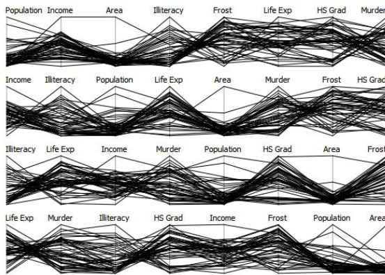
Figure 12: Different axis orders exhibit different patterns of correlation. The 8-dimensional census dataset [BCW88] shows several statistics of the 50 states of the United States of America and is layed out in the parallel coordinates matrix (PCM) [HSW12] such that every pair of axes appears exactly once. The topmost plot shows a negative correlation between “Illiteracy” and “Frost”, while the bottom plot indicates that “Life Exp” is negatively correlated with “Murder”. Taking a close look at the “HS Grad” axes, we find that there is a cluster of states having a low rate of high-school graduates. Also, the bottom row indicates a negative correlation between “Illiteracy” and “HS Grad”. A moderately negative correlation seems to be between “Life Exp” and “Illiteracy” in the third row, as well as a positive correlation with “Income”.
