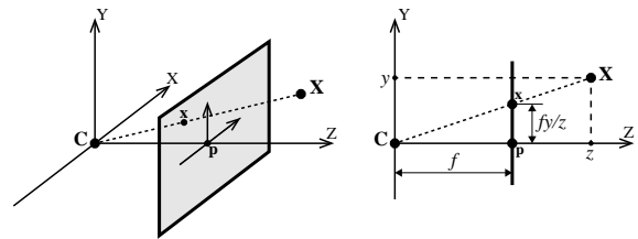
Figure 3: Camera geometry: (left) \mathbf{C} denoted the camera center and \mathbf{p} the principal point. In a basic setup the center of the first camera is centered at the origin; (right) 2d cross section of the projection.
