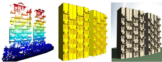
Figure 12: Results of interactive fitting of “SmartBoxes” to uncomplete LiDAR data. Figure courtesy of Liangliang Nan [NSZ*10], ©2010 ACM.
