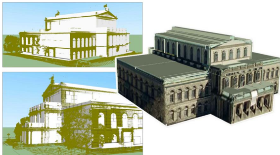
Figure 14: Automatic reconstruction of a building with volumetric models. For purposes of visual evaluation, the reconstructed volume is superimposed over the original point set, including noise and obstacles (left), and textured with photographs of the buildings (right). Figure courtesy of Carlos Vanegas [VAB12], ©2012 IEEE.
