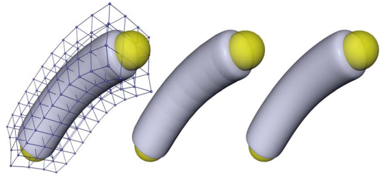
Figure 4: Comparison between tri-linear (middle) and B-Spline (right) interpolation.
