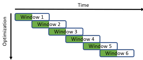
Figure 5: To provide enough far-sightedness while still keeping the dimensionality feasible, the optimization considers a shorter control window containing only a few offset poses. Using overlapping control windows allows to take goals of the next window into account which ensures good initial conditions for the next window.
