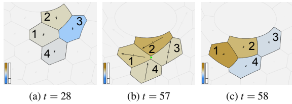
Figure 1: Topological change. We show three different time steps (in the sedimenting-ellipse simulation), bubbles color-mapped by pressure and velocity shown using arrows. In Fig. 1a bubble edges meet 3-way, with bubbles 1 and 3 adjacent (we choose t=28 as opposed to t=56 to emphasize the evolution of the four bubbles). As the falling ellipse compresses the bubbles, the film shared by bubbles 1 and 3 decreases in length (Fig. 1b), until the four bubbles move to an unstable configuration in which edges meet 4-way. Note the high velocity that bubbles have after the topological change. Fig. 1c shows the four bubbles after the topological change where bubbles 2 and 4 are adjacent, and edges meet 3-way.
