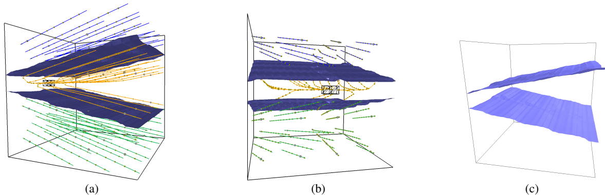
Figure 11: Separatrices found using inflow/outflow enhancement in the critical point data set. Streamlines can have one of three different entrance properties, however, they all have the same exit property. Figures (a) and (b) show streamlines in addition to the separatrices. The critical point is located on the shared diagonal of the tetrahedra outlined in black. Figure (c) shows the separatrices that would not have been generated by the original algorithm.
