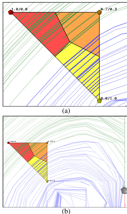
Figure 2: Sampling with streamlines and tabulating their values. Figure (a) shows a close-up view of a cell in a 2D data set. The Voronoi cell decomposition is shown to illustrate tabulation assignments (e.g. all portions of the streamlines that are in the red section of the cell contribute to the red vertex). The accumulated properties are also shown, on a per-vertex basis. Thus the red vertex has 100% contribution from the green streamlines, the yellow vertex has 100% contribution from the blue streamlines and the orange vertex has 70% green contribution and 30% blue contribution. Figure (b) shows the cell embedded in the data set. Notice the green streamlines accumulate their properties from the green section of the boundary, while the blue streamlines are accumulating their properties from an internal “orbit.”
