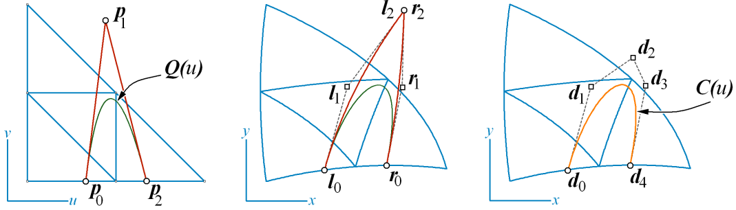
Figure 7: Relationship between control net of Q(u) and control net of C(u) . Left image shows rational-quadratic curve Q(u) in parameter space. Middle image shows control net of Q(u) transformed into physical space. Right image shows rational-quartic curve C(u) resulting from transforming Q(u) into physical space. It turns out that l_1 = d_1 , r_1 = d_3 , T(p_0) = d_0 , and T(p_2) = d_4 .
