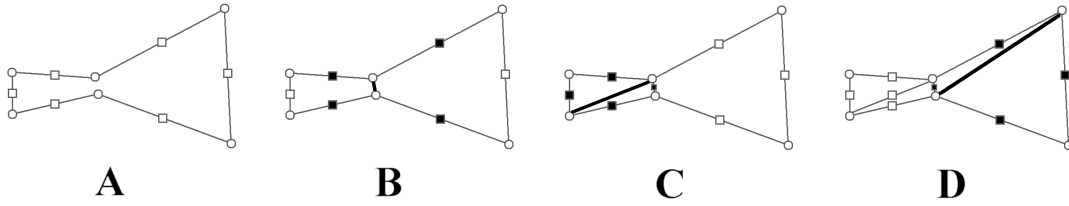
Figure 6: Constructing four triangular patches from six face-intersection curves. Circles are endpoints and squares are center control points of face-intersection curves. Dark lines are chosen diagonal for splits. Dark squares are control points used to determine the center control point for each diagonal. An original polygon is shown in image A. Image B shows the first diagonal selection. Image C shows the diagonal selection for the left half. Image D shows the diagonal selection for the right half.
