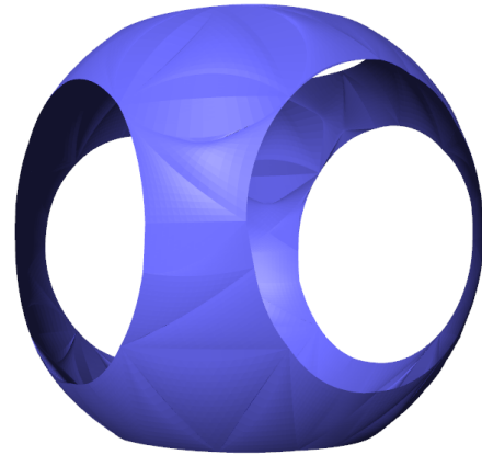
Figure 9: Enlargement of rational-quartic contour surface extracted from un-twisted mesh shown in Figure 8 (left); 320 quadratic tetrahedra.
