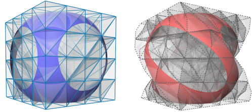
Figure 8: Left image shows “un-twisted” mesh containing only linear-edge quadratic tetrahedra. Right image shows twisted mesh containing curved-quadratic tetrahedra. The mesh is twisted by 90° comparing top and bottom faces of entire mesh configuration.
