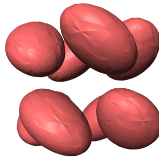
Figure 12: Rational-quartic contour surface extracted from 15918 curved-quadratic tetrahedra.
