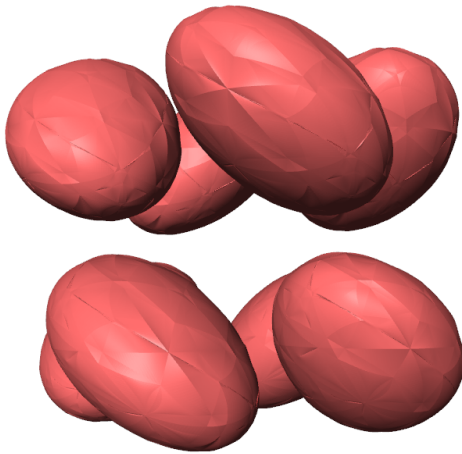
Figure 12: Rational-quartic contour surface extracted from 15918 curved-quadratic tetrahedra.
