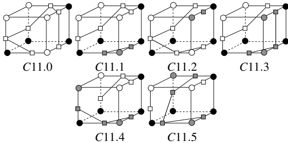
Figure 11: Sub-cases for topology base case C11.
