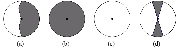
Figure 1: (a) Around a regular point \mathbf{x} \in \mathbb{R}^3 , the isosurface F^{-1}(F(\mathbf{x})) divides space into a single connected volume P with F > 0 (dark gray) and a single connected volume N with F < 0 (white). (b)/(c) Around a minimum/maximum, all points in U have a larger/smaller value than F(\mathbf{x}) . (d) In case of a saddle, there are multiple (more than one) regions with values larger or smaller than the value F(\mathbf{x}) .
