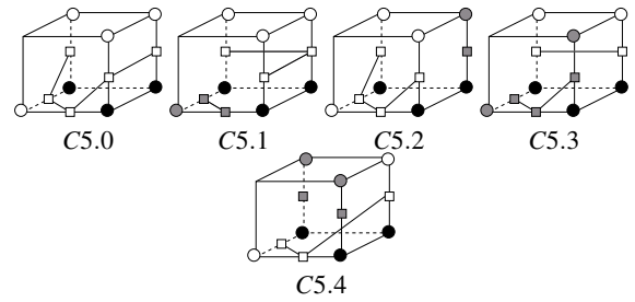
Figure 8: Sub-cases for topology base case C5.
