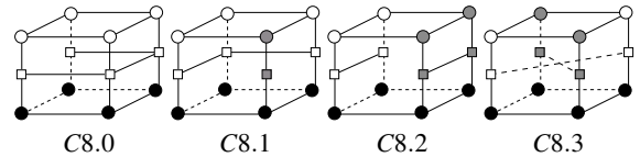
Figure 9: Sub-cases for topology base case C8.
